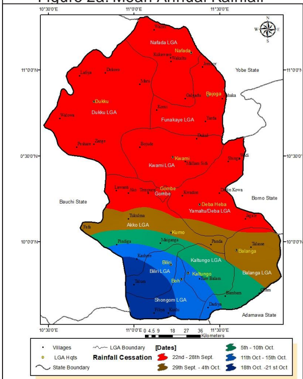
Figure 2c. Rainfall Cessation
