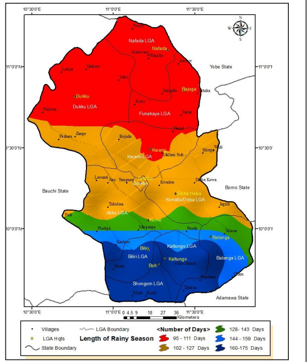
Figure 2d. Length of Rainy Season
