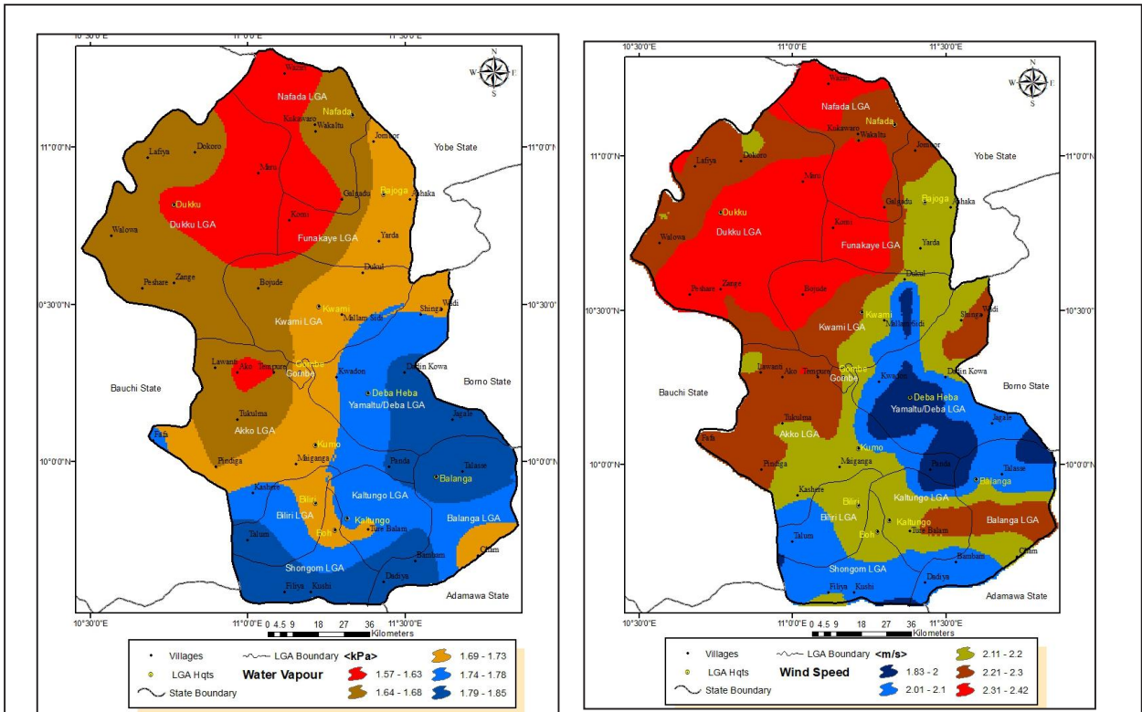
Figure 6b, Wind Speed
