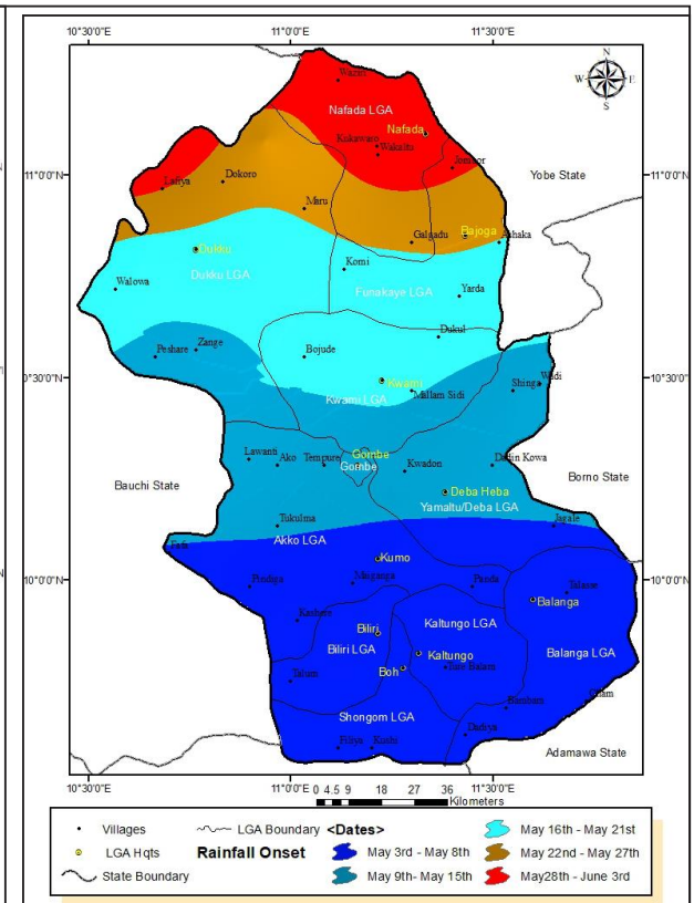
Figure 2b. Rainfall Onset
